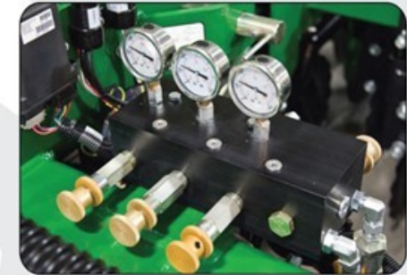
HYDRAULIC WEIGHT TRANSFER - Ensures that all rows have the same amount of weight available for penetration - even when crossing undulations.
