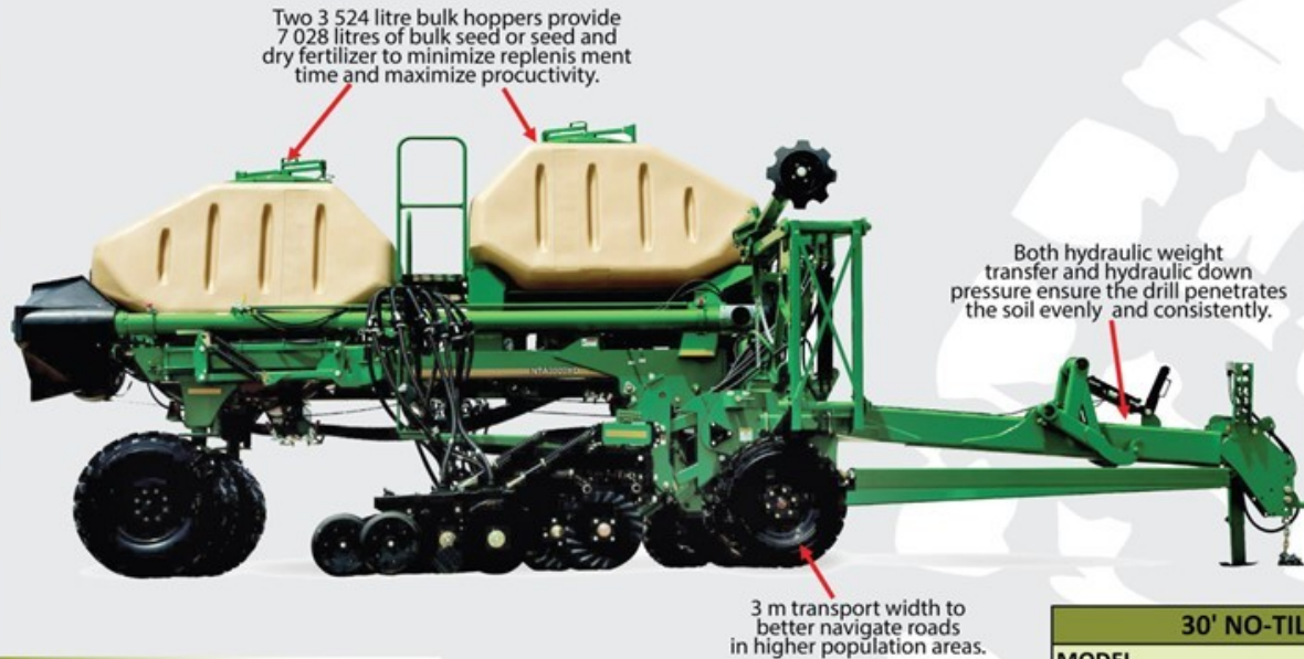
HYDRAULIC WEIGHT TRANSFER - Ensures that all rows have the same amount of weight available for penetration - even when crossing undulations.
